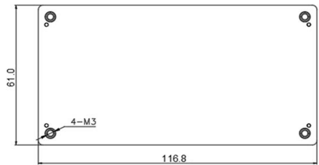
Standard 116.8x61.0x12.7 mm
