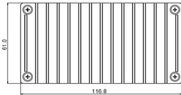
Standard+Heatsink 116.8x61.0x32.7 mm
