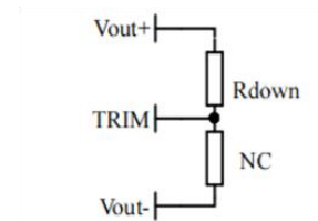
Voltage-down: Add R_{down} between Trim and Vout+
