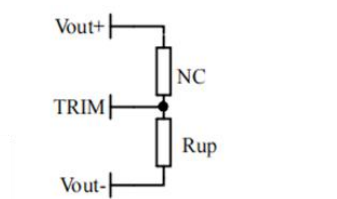
Voltage-up: Add R_{up} between Trim and Vout-
