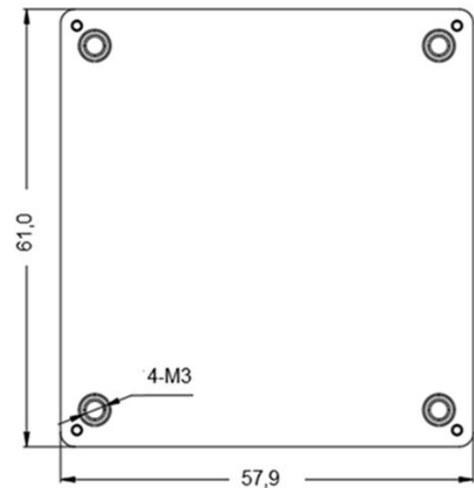
Standard 61.0x57.9x12.7mm
