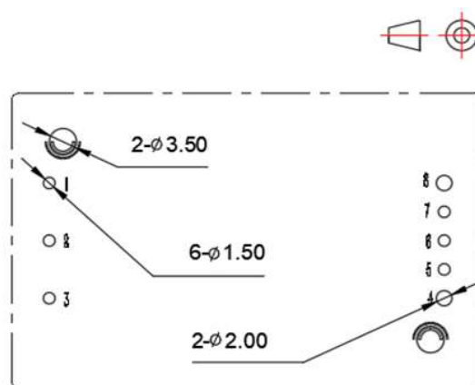
Recommended PCB holes size
