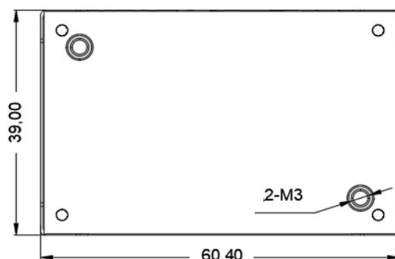
Standard 60.4x39.0x12.7mm
