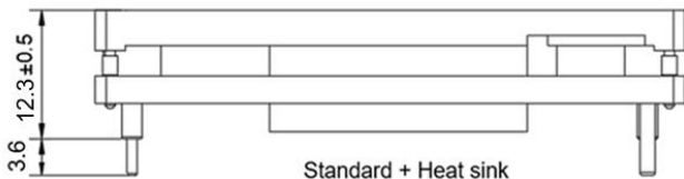
Standard + Heat sink 58.1mmX23.0mmX12.3mm
